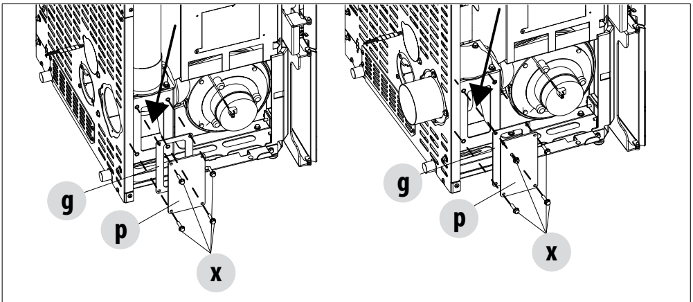
CLEANING TOP SMOKE OUTLET
